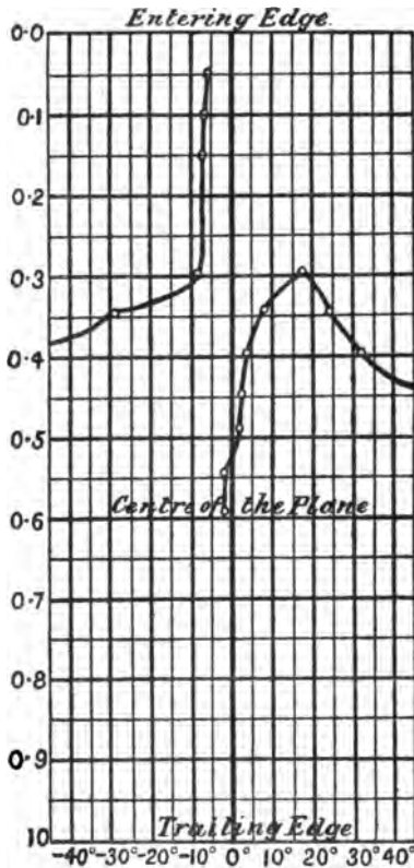
FIG. 30.—Angles i of the chord and the wind, and distribution of the pressure itself, but only the point at which its effect is applied to the plane, this point being known as the centre of pressure .
